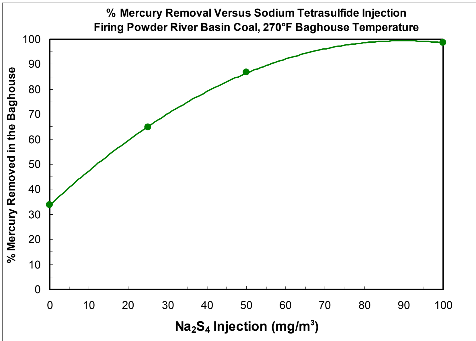
Figure 5. Mercury removal by injecting sodium tetrasulfide at the baghouse while firing PRB coal.
